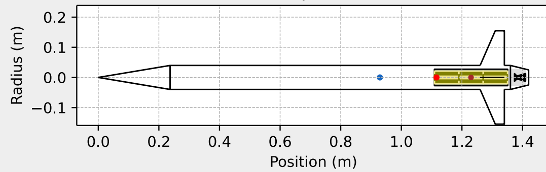
Rocket Representation
